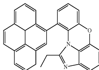
[Chemical Formula 1-8-29]
