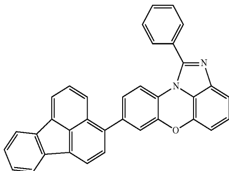
[Chemical Formula 1-4-30]
