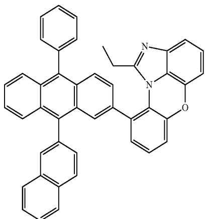
[Chemical Formula 1-8-23]
