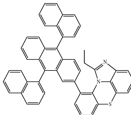
[Chemical Formula 2-3-21]
