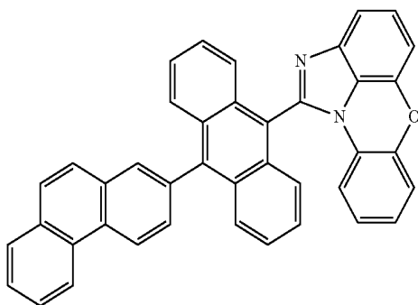
[Chemical Formula 1-1-17]
