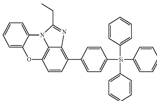
[Chemical Formula 1-11-13]
