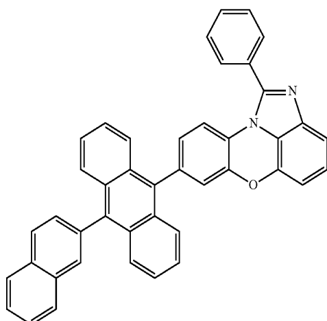
[Chemical Formula 1-4-2]
