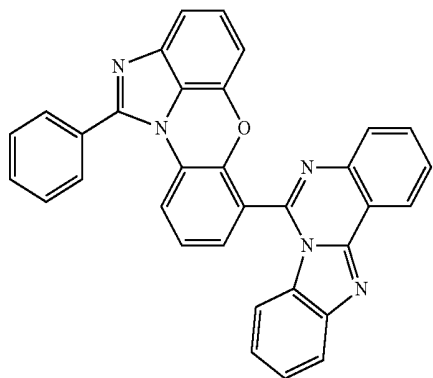
[Chemical Formula 1-6-54]
