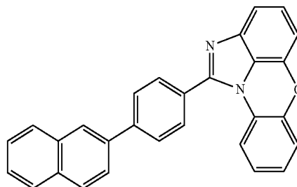
[Chemical Formula 1-1-35]
