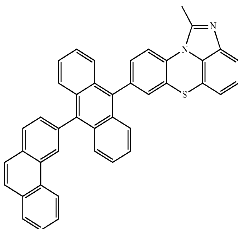
[Chemical Formula 2-2-8]
