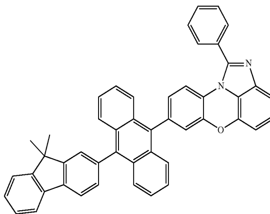
[Chemical Formula 1-4-5]
