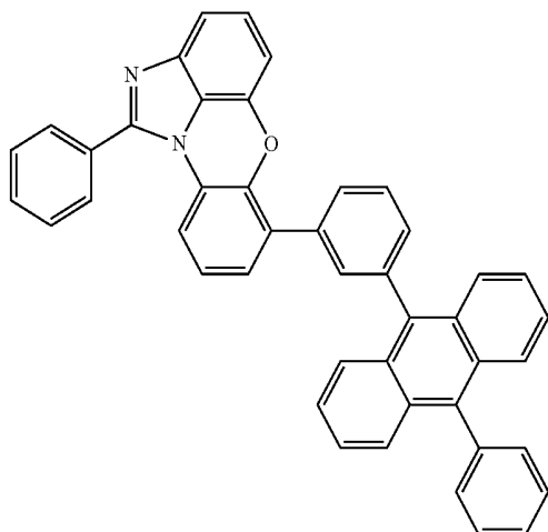
[Chemical Formula 1-6-18]
