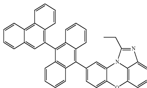
[Chemical Formula 1-7-8]
