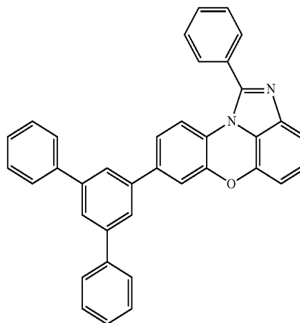
[Chemical Formula 1-4-40]
