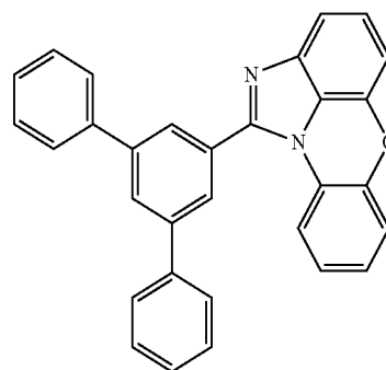
[Chemical Formula 1-1-48]
