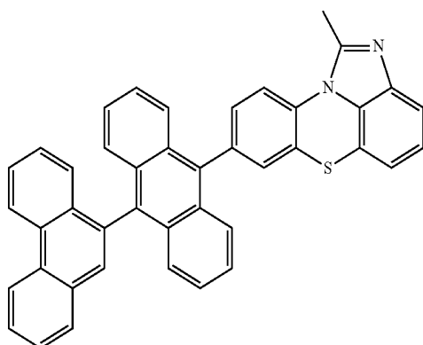
[Chemical Formula 2-2-7]
