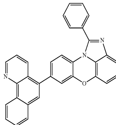
[Chemical Formula 1-4-34]
