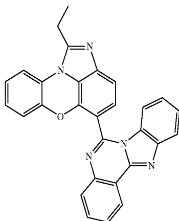
[Chemical Formula 1-9-17]
