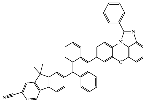
[Chemical Formula 1-4-15]
