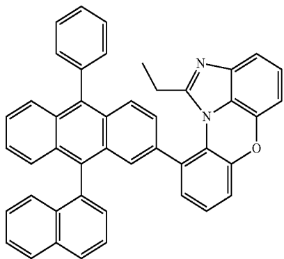
[Chemical Formula 1-8-22]
