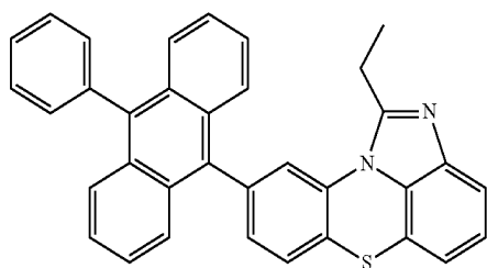
[Chemical Formula 2-3-1]
