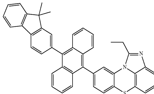
[Chemical Formula 2-3-6]
