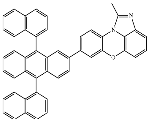
[Chemical Formula 1-2-21]
