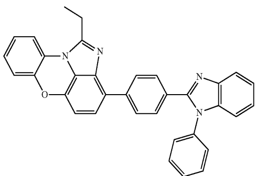
[Chemical Formula 1-11-9]
