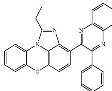
[Chemical Formula 1-11-14]
