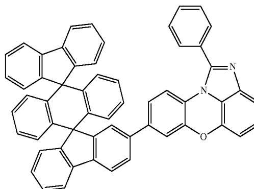
[Chemical Formula 1-4-36]
