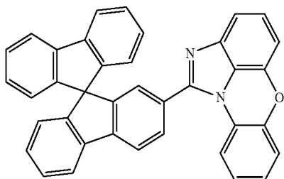
[Chemical Formula 1-1-42]
