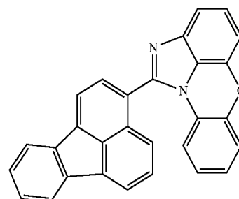
[Chemical Formula 1-1-38]
