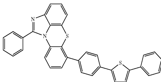
[Chemical Formula 2-2-39]
