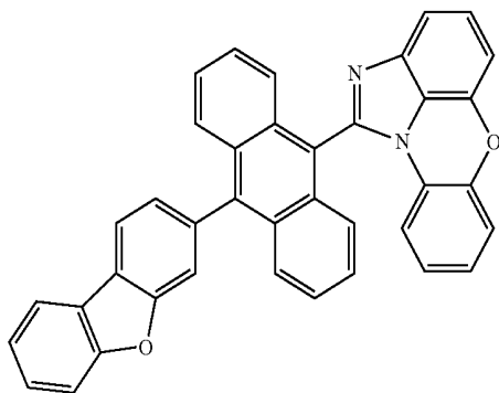
[Chemical Formula 1-1-21]
