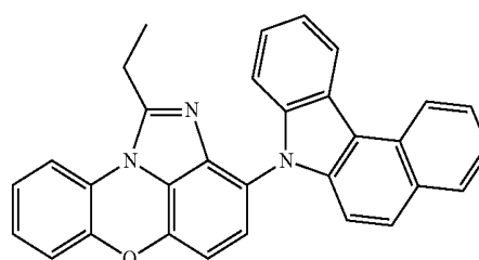
[Chemical Formula 1-11-15]
