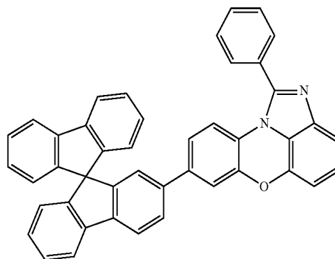
[Chemical Formula 1-4-35]
