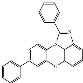
[Chemical Formula 1-4-37]
