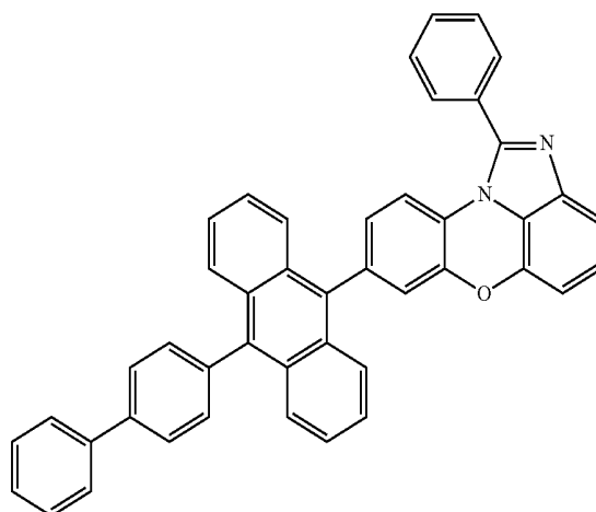
[Chemical Formula 1-4-4]
