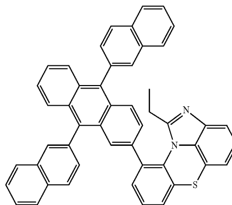
[Chemical Formula 2-3-20]
