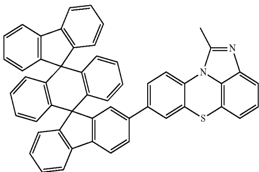
[Chemical Formula 2-2-36]
