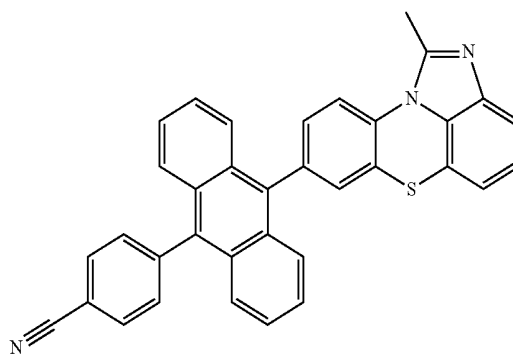
[Chemical Formula 2-2-12]
