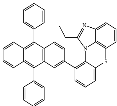
[Chemical Formula 2-3-19]
