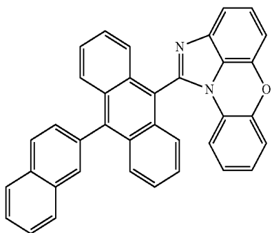
[Chemical Formula 1-1-10]
