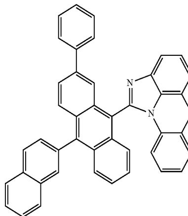
[Chemical Formula 1-1-25]
