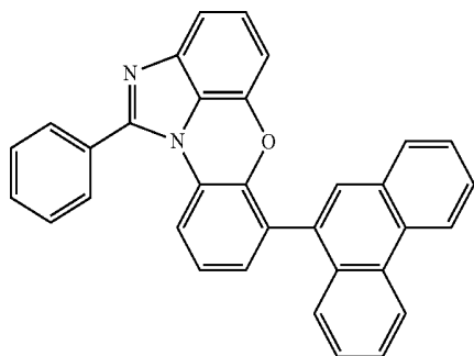
[Chemical Formula 1-6-31]
