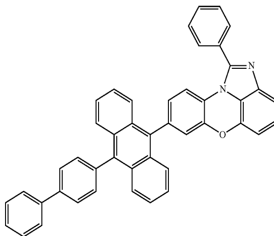
[Chemical Formula 1-4-4]
