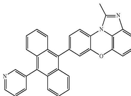
[Chemical Formula 1-2-10]
