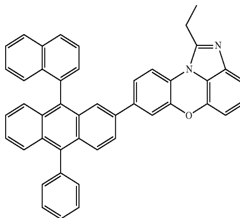
[Chemical Formula 1-3-22]
