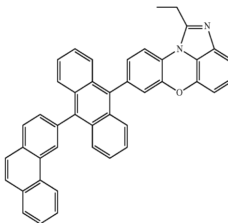
[Chemical Formula 1-3-8]
