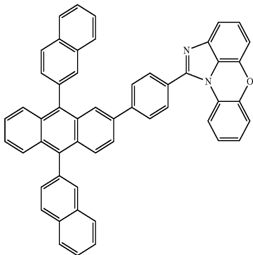
[Chemical Formula 1-1-33]
