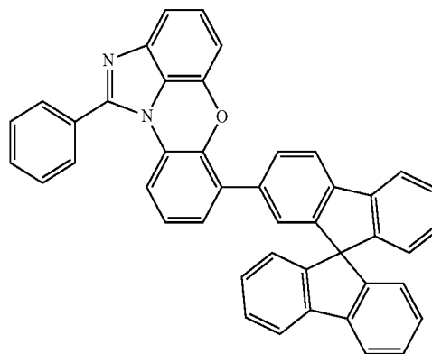
[Chemical Formula 1-6-35]
