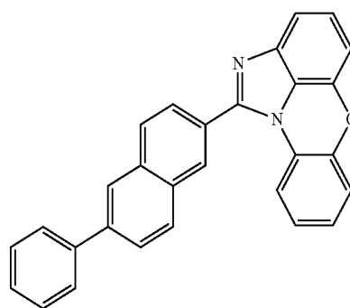
[Chemical Formula 1-1-36]
