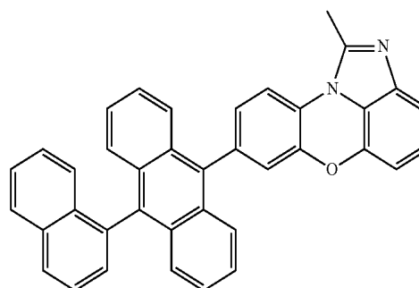
[Chemical Formula 1-2-3]
