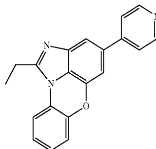
[Chemical Formula 1-9-16]
