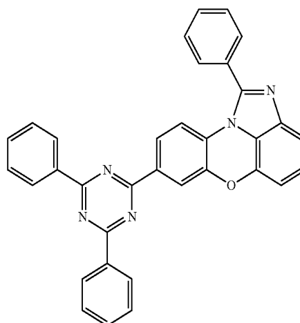
[Chemical Formula 1-4-41]
