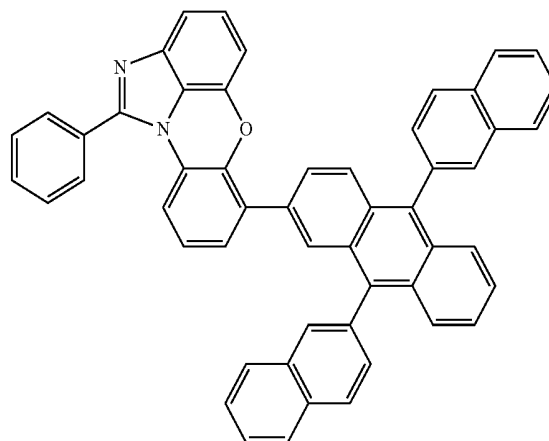
[Chemical Formula 1-6-20]
