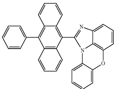
[Chemical Formula 1-1-9]
