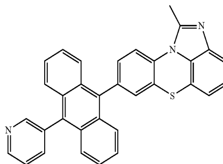
[Chemical Formula 2-2-10]
