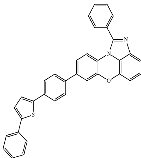
[Chemical Formula 1-4-39]
