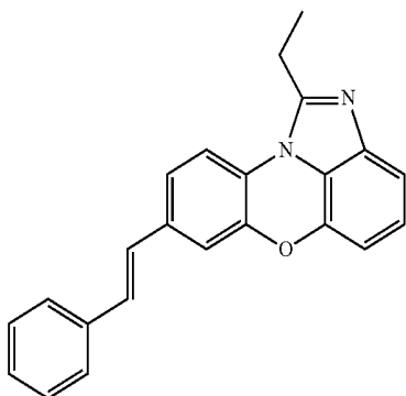
[Chemical Formula 1-3-54]
