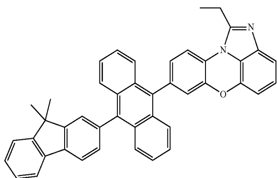
[Chemical Formula 1-3-5]
