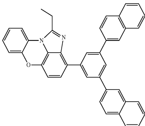
[Chemical Formula 1-11-7]
