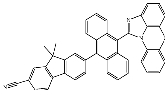
[Chemical Formula 1-1-23]
