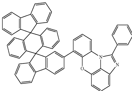
[Chemical Formula 1-6-36]
