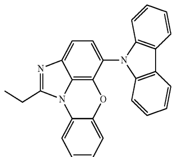
[Chemical Formula 1-9-14]
