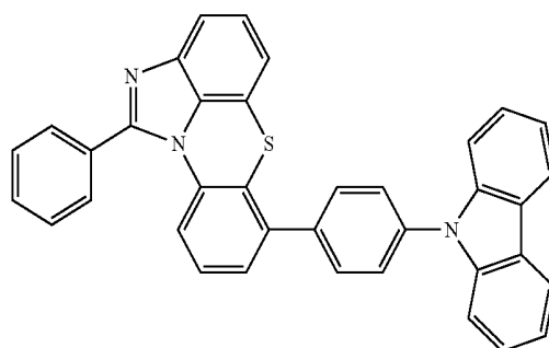
[Chemical Formula 2-2-42]
