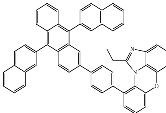
[Chemical Formula 1-8-26]
