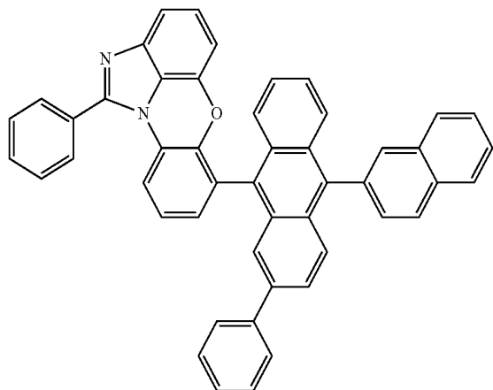
[Chemical Formula 1-6-16]
