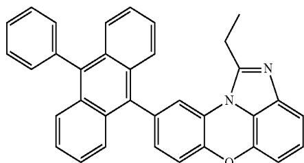
[Chemical Formula 1-7-2]
