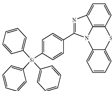
[Chemical Formula 2-1-8]
