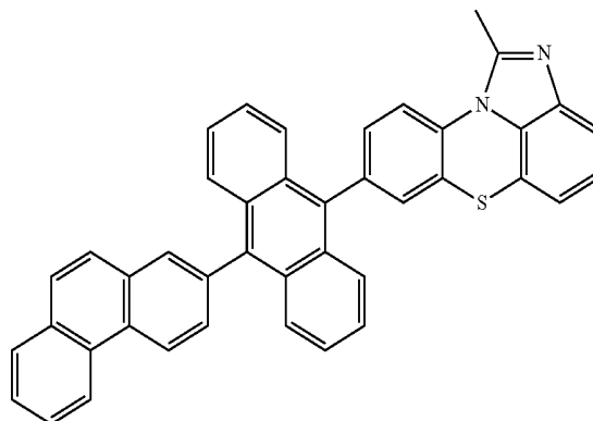
[Chemical Formula 2-2-9]
