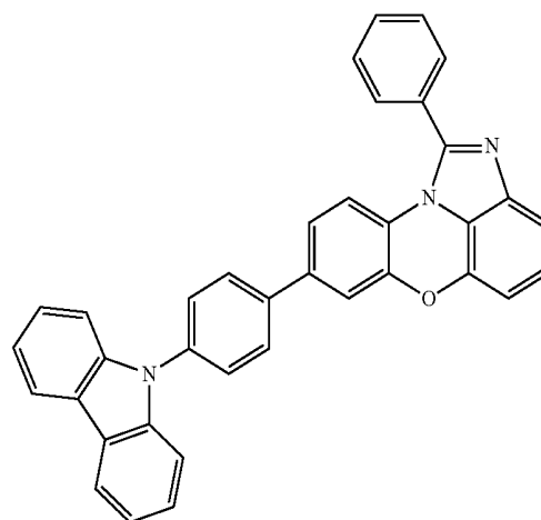
[Chemical Formula 1-4-42]
