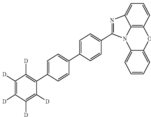
[Chemical Formula 1-1-61]
