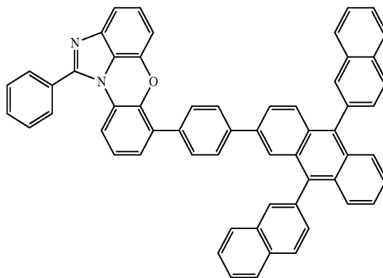
[Chemical Formula 1-6-25]
