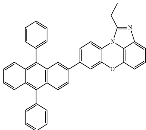
[Chemical Formula 1-3-19]
