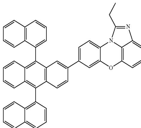
[Chemical Formula 1-3-21]
