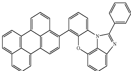
[Chemical Formula 1-6-29]
