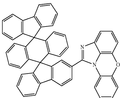
[Chemical Formula 1-1-45]
