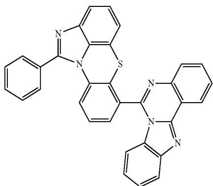
[Chemical Formula 2-2-54]
