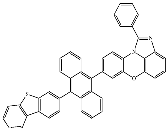
[Chemical Formula 1-4-14]
