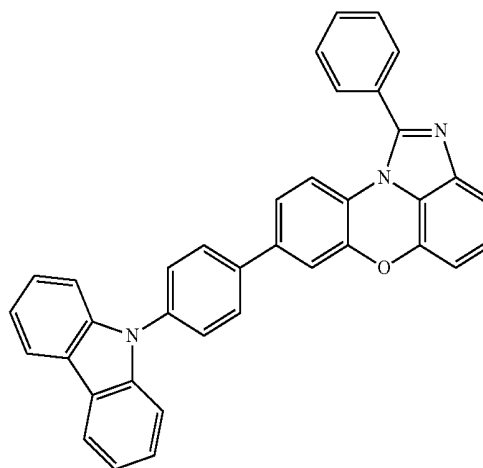
[Chemical Formula 1-4-42]
