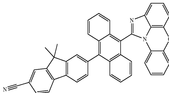
[Chemical Formula 1-1-23]
